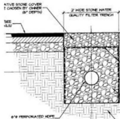
UNDERGROUND PIPING
